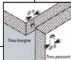
Trou passant
